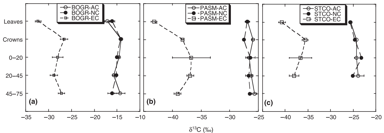
Fig. 5 \delta^{13}\text{C} values in leaves, crowns, and roots at 3 depths after 5 yrs of experimental treatments in the three most abundant grasses.
